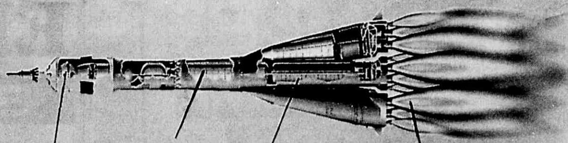
The Rocket carried its own oxygen in this tank
